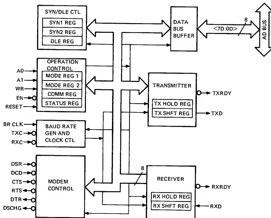
Figure 2-4 2651 USART
